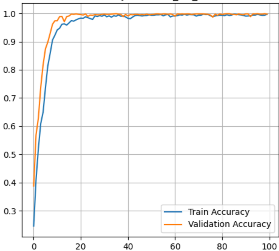
Accuracy: FCovSel_SG_MSC
